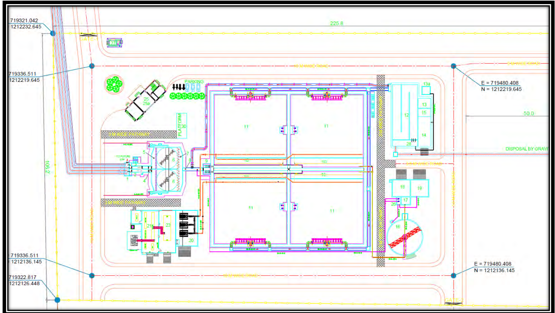
Figure 4: Sewage Treatment Plant Layout Map
